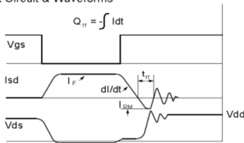
Diode Recovery Test Circuit & Waveforms
