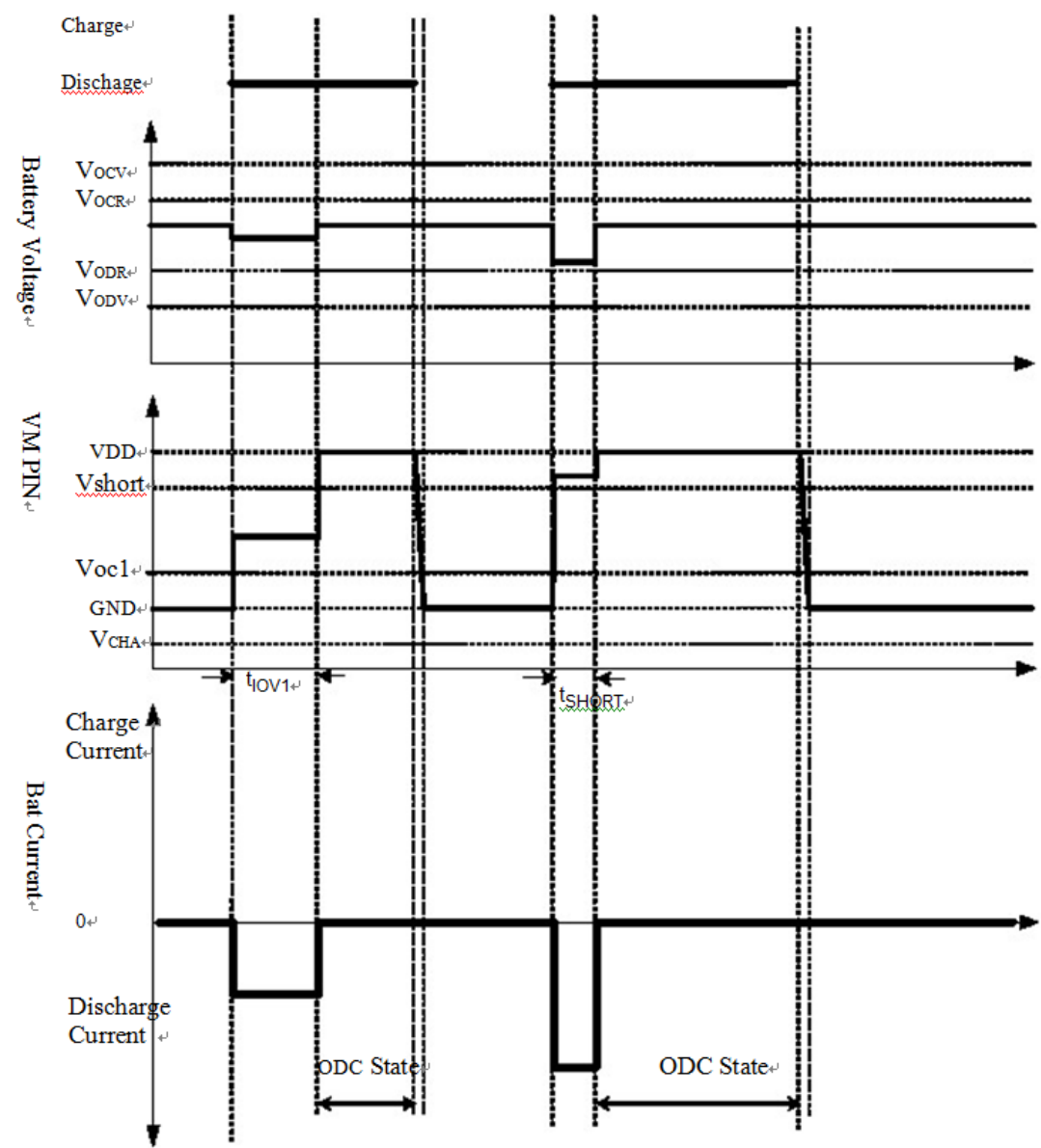
Figure 6. Over Discharge current and Normal state timing
