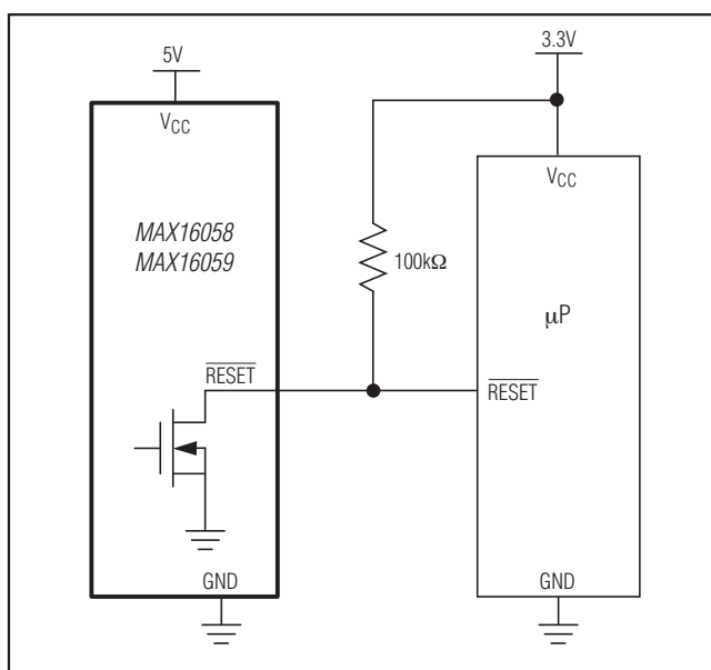
Figure 5. Interfacing with Other Voltage Levels
