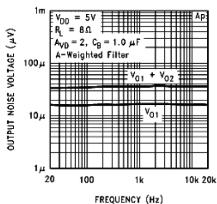
Noise Floor
