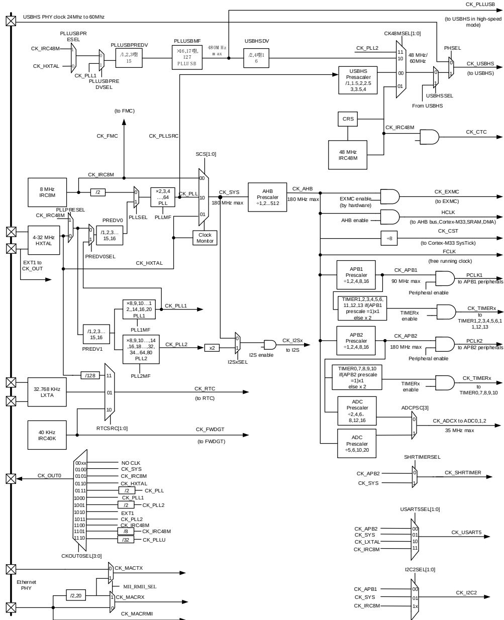
Figure 2-5. GD32A508xx clock tree
