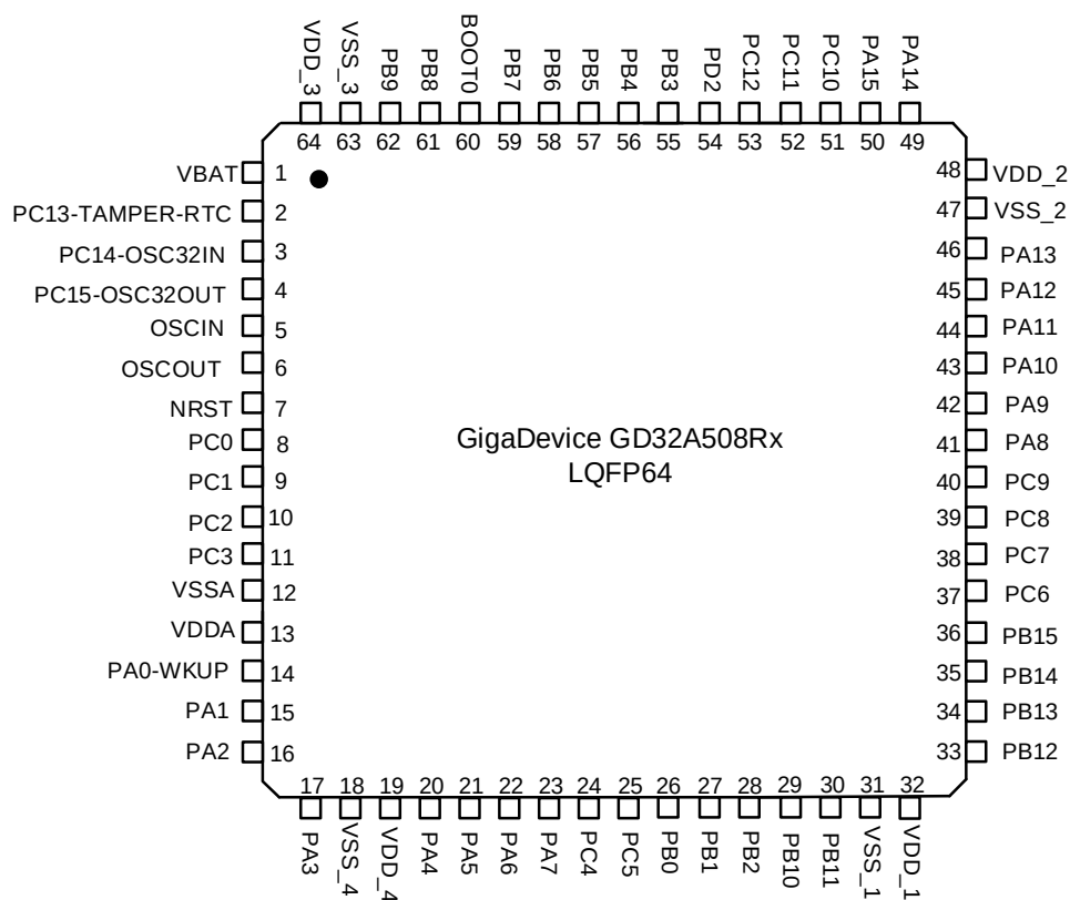
Figure 2-4. GD32A508Rx LQFP64 pinouts
