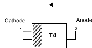
Simplified outline SOD-323 and symbol
