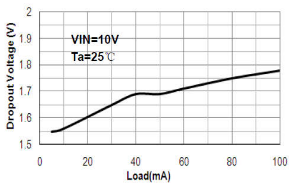
Dropout Voltage vs. Load
