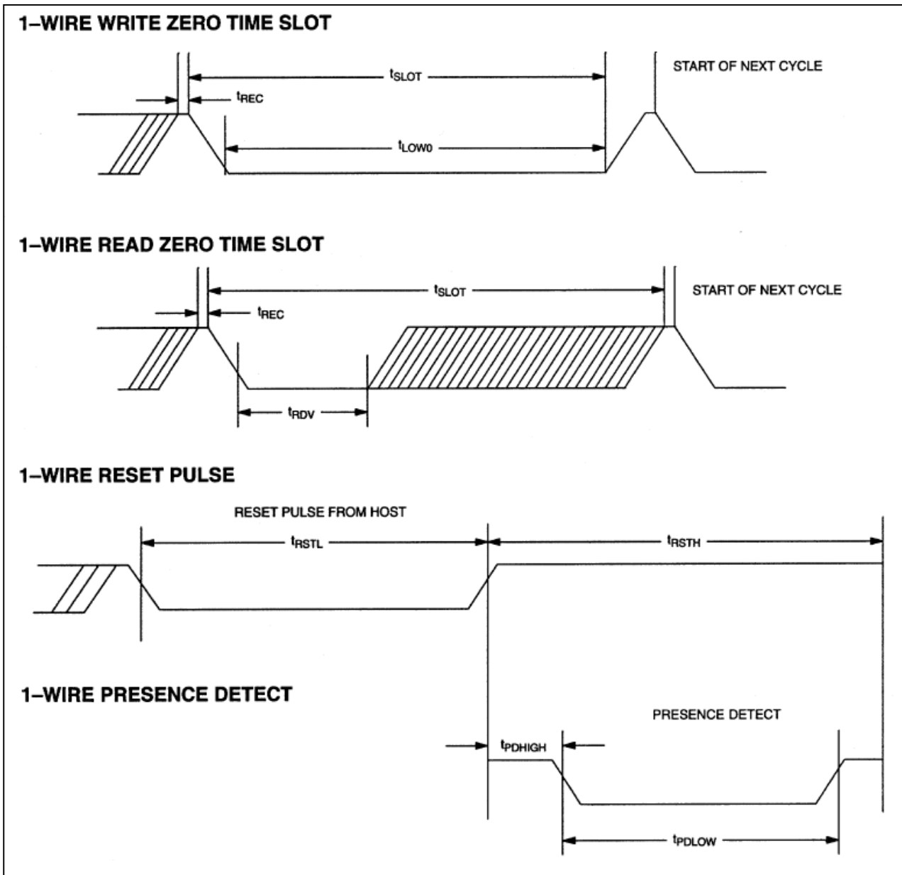
Figure 18. Timing Diagrams
