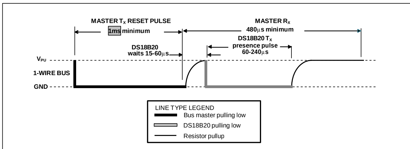
Figure 13. Initialization Timing
