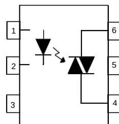
Pin Configuration
