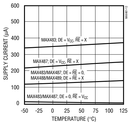
MAX483/MAX487-MAX489 SUPPLY CURRENT vs. TEMPERATURE
