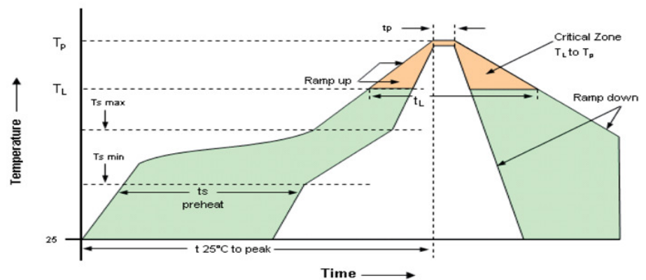
Solderprofile:
