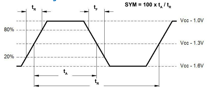
Fig 2: LVPECL Waveform
