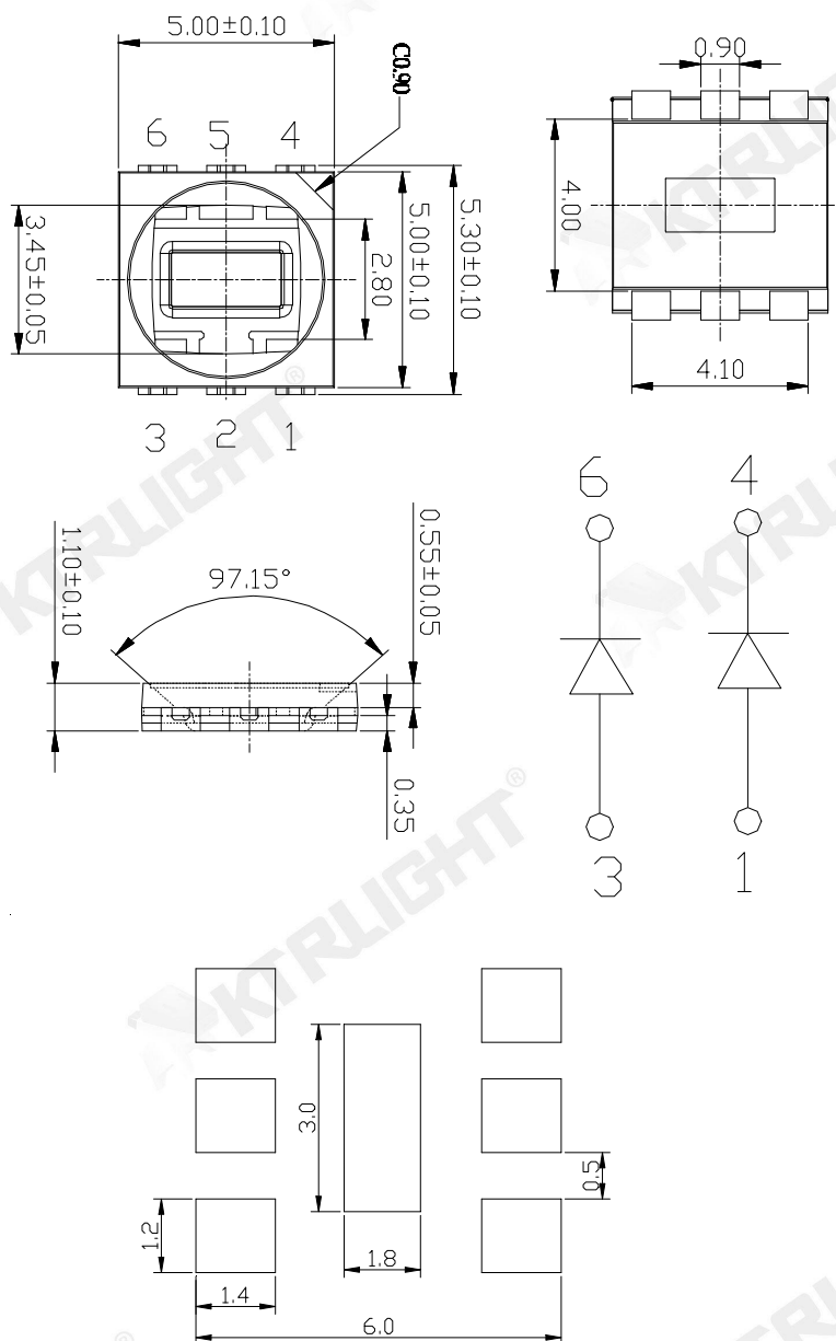
推荐焊盘式样(Recommended Soldering Patter)
