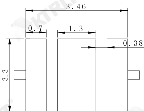
推荐焊盘式样(Recommended Soldering Patter)
