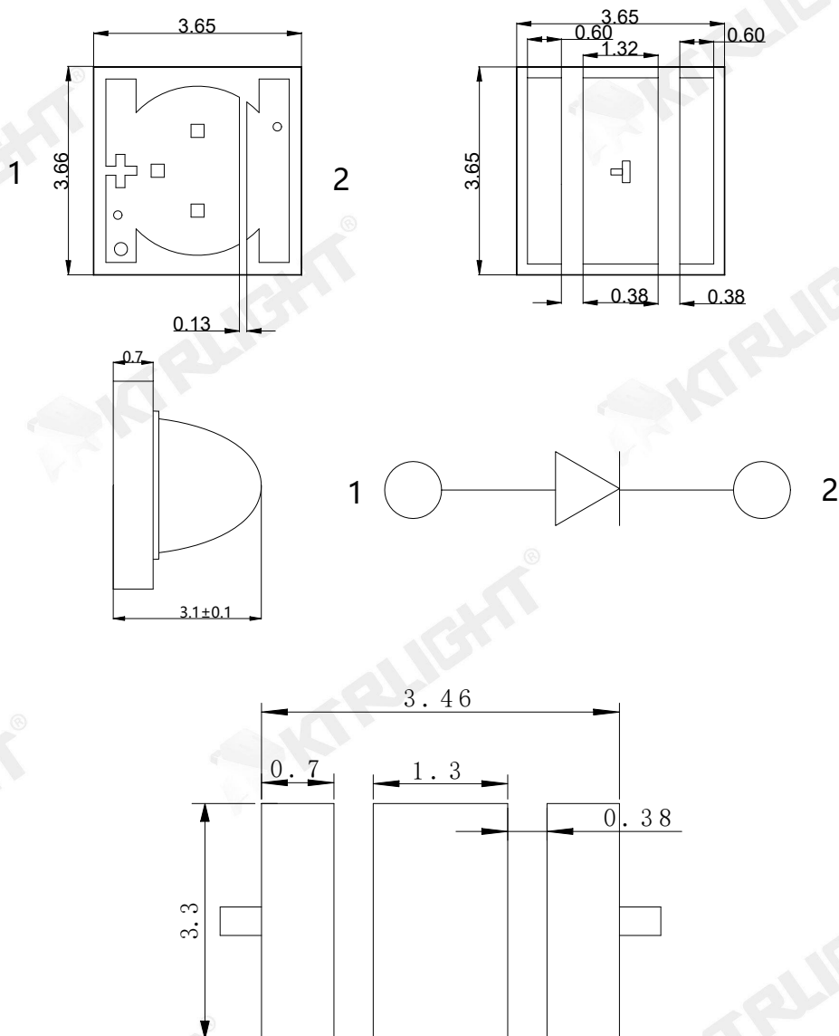
推荐焊盘式样(Recommended Soldering Patter)
