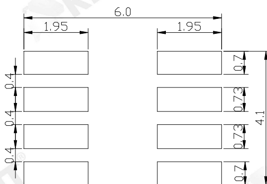
推荐焊盘式样(Recommended Soldering Patter)
