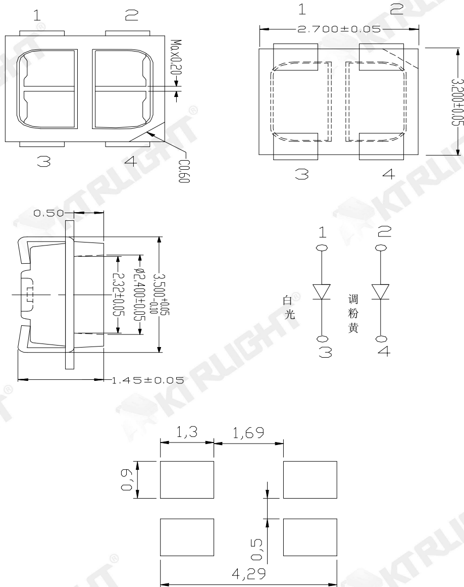
推荐焊盘式样(Recommended Soldering Patter)
