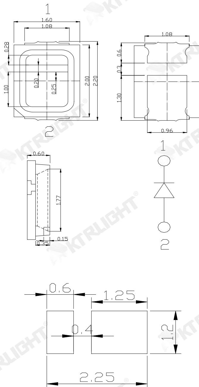
推荐焊盘式样 (Recommended Soldering Patter)
