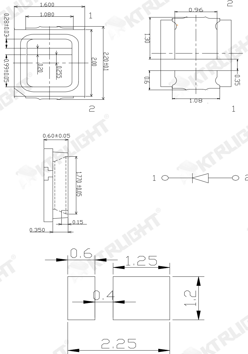
推荐焊盘式样(Recommended Soldering Patter)
