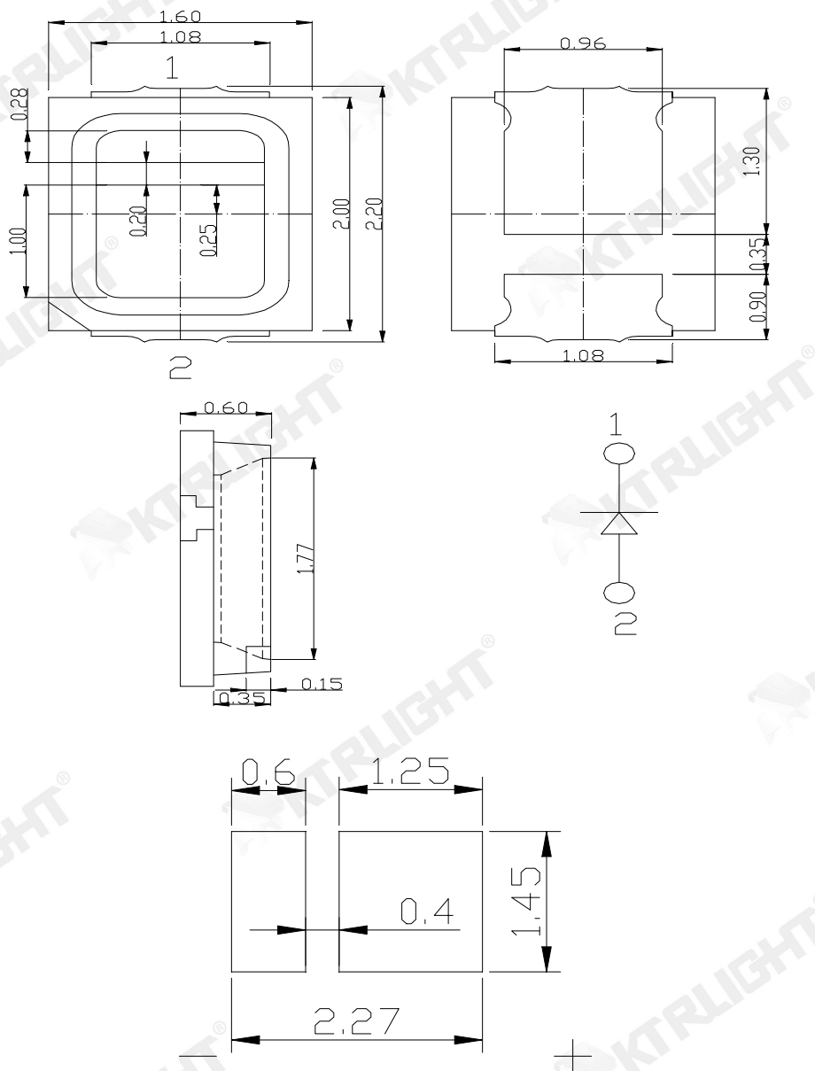
推荐焊盘式样 (Recommended Soldering Patter)
