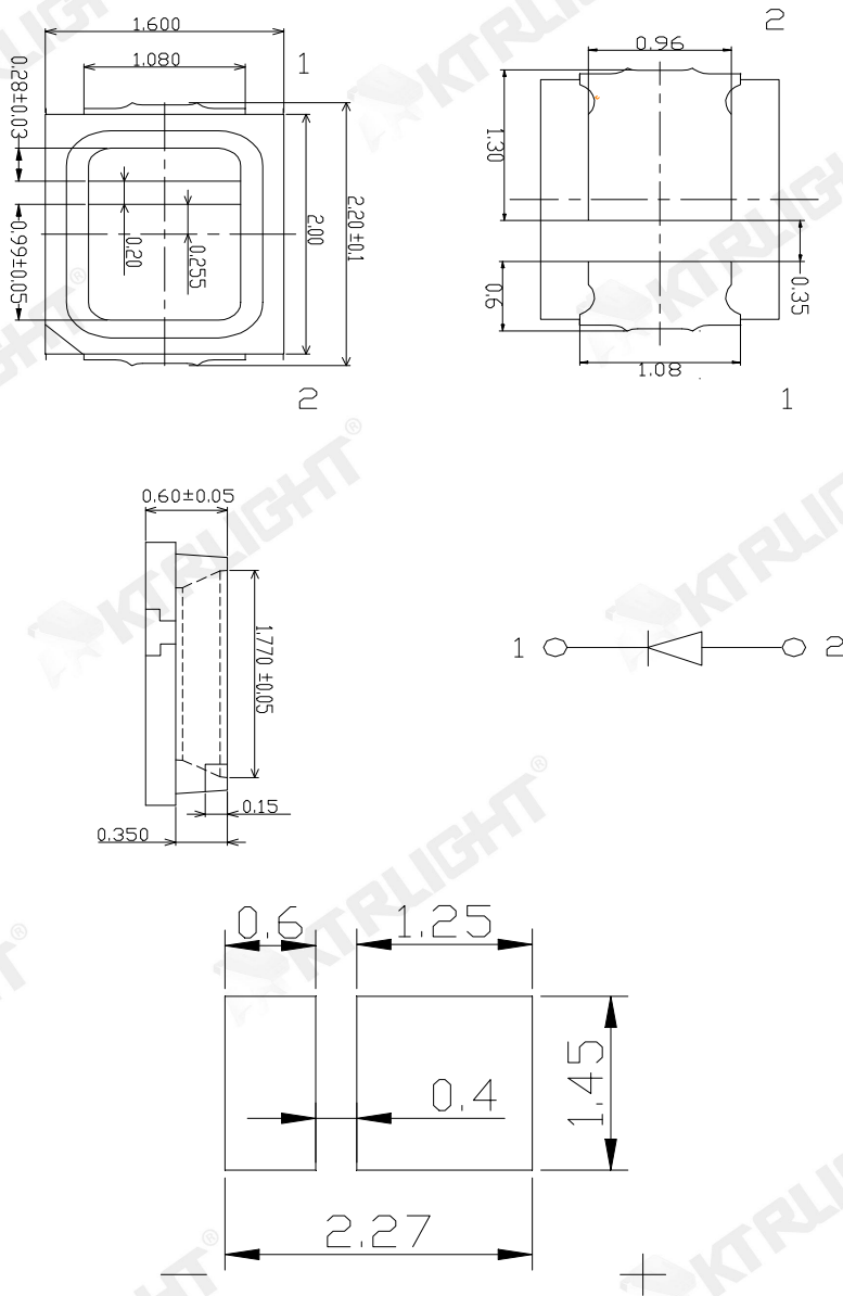
推荐焊盘式样(Recommended Soldering Patter)
