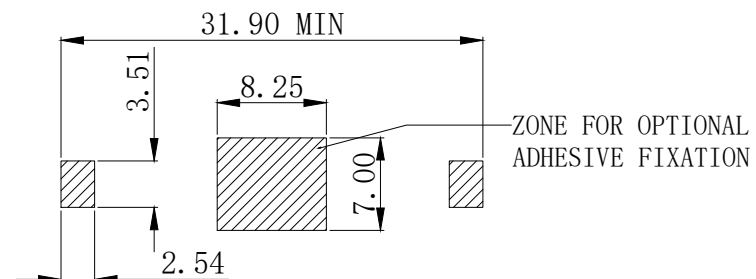
PCB LAYOUT
