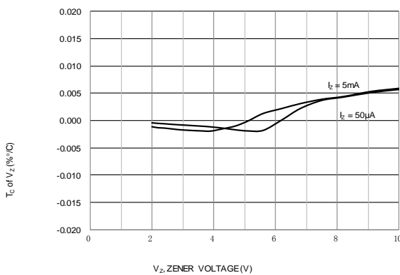
Fig. 5 Typical Temperature Coefficient of Zener Voltage
