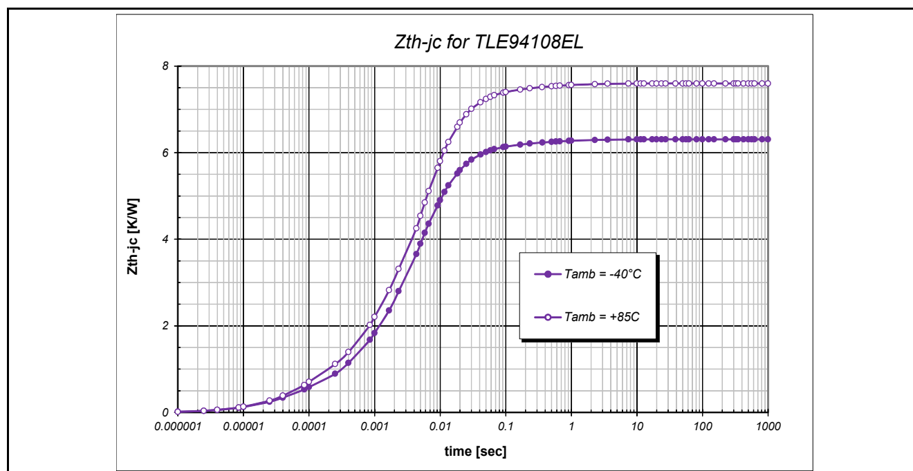
Figure 30 ZthJC Curve
