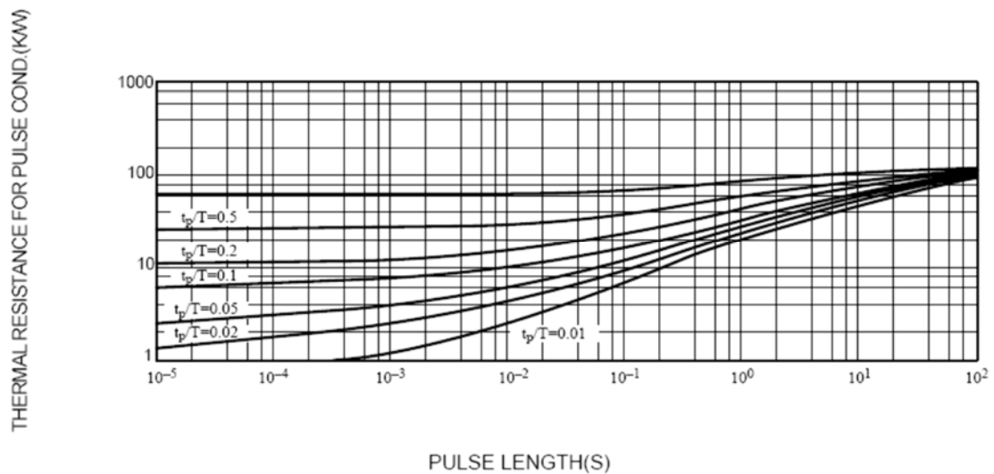
FIG.3 – THERMAL RESPONSE
