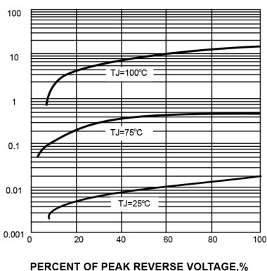
FIG. 4-TYPICAL REVERSE CHARACTERISTICS
