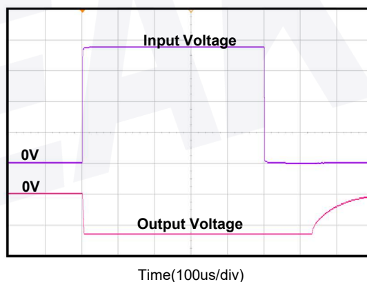
Inverting Differential Input Overload
