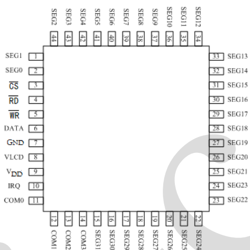
QFP44
