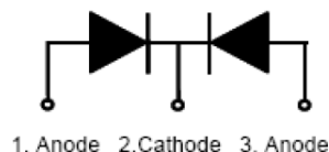
Package: TO-220-AB SBR10100CT
