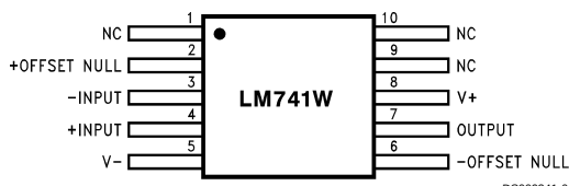
Ceramic Flatpak
