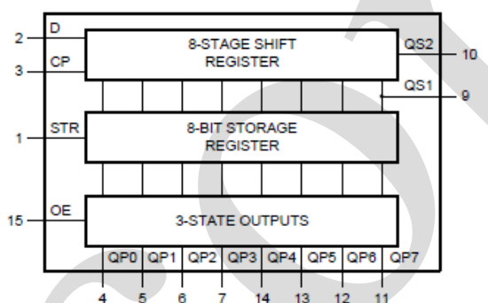
Figure 2. Functional diagram
