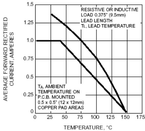
FIG. 1 - FORWARD CURRENT DERATING CURVES
