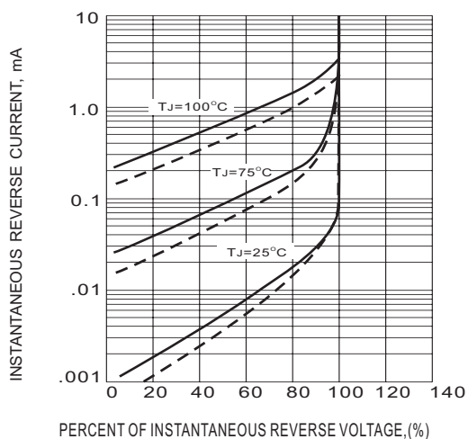
Fig.3-TYPICAL REVERSE CHARACTERISTIC
