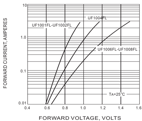
Fig.3 FORWARD CHARACTERISTICS
