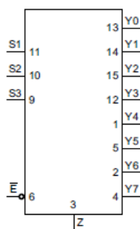
Figure 1. Logic symbol
