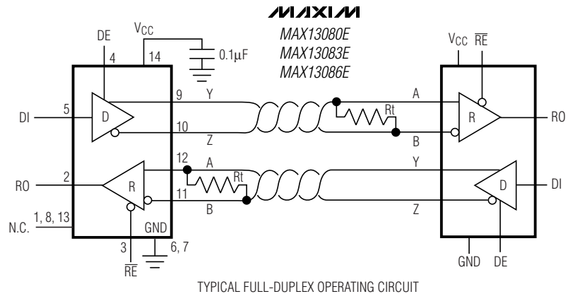
TYPICAL FULL-DUPLEX OPERATING CIRCUIT
