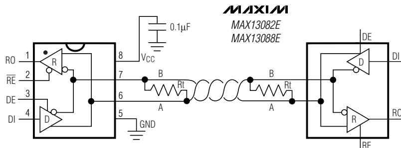
TYPICAL HALF-DUPLEX OPERATING CIRCUIT
