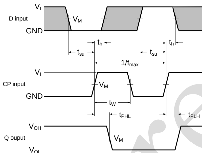
Figure 6. Clock (CP) to output (Q) propagation delay times, clock pulse width, D to set-up times, the CP to D hold times and maximum clock pulse frequency
