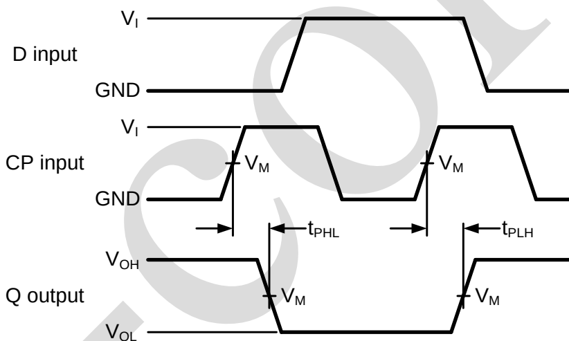
Figure 5. Clock (CP) to output (Q) propagation delay times
