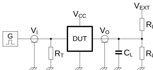
Figure 4. Test circuit for measuring switching times
