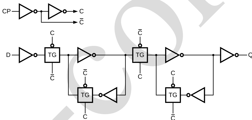
Figure 3. Logic diagram
