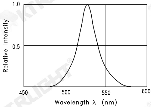
Fig.1 RELATIVE INTENSITY VS. WAVELENGTH
