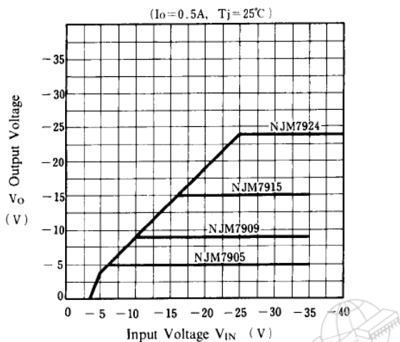
NJM7900 Output Characteristics
