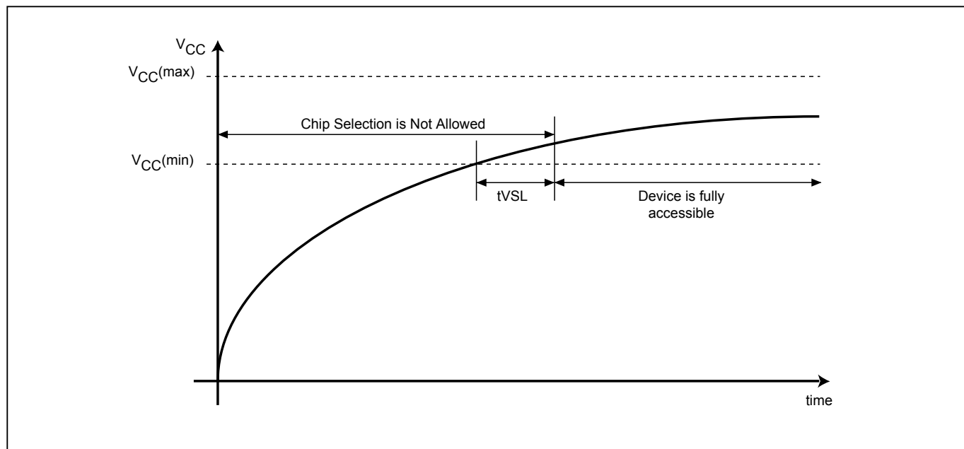
Figure 28. Power-up Timing
