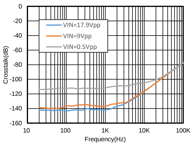
V_S = \pm 15V , V_{CM} = 0V Figure 29. Crosstalk vs. Frequency
