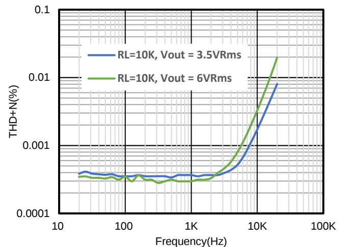
V_S = \pm 15V , V_{CM} = 0V , G = 1 Figure 28. THD+N vs. Frequency
