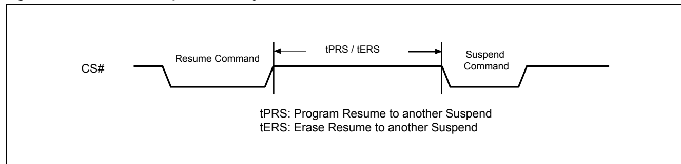
Figure 33. Resume to Suspend Latency
