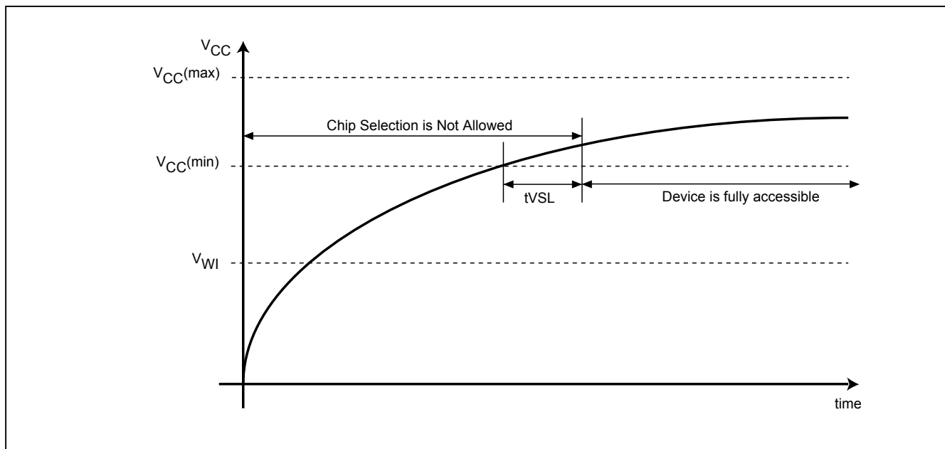
Figure 48. Power-up Timing
