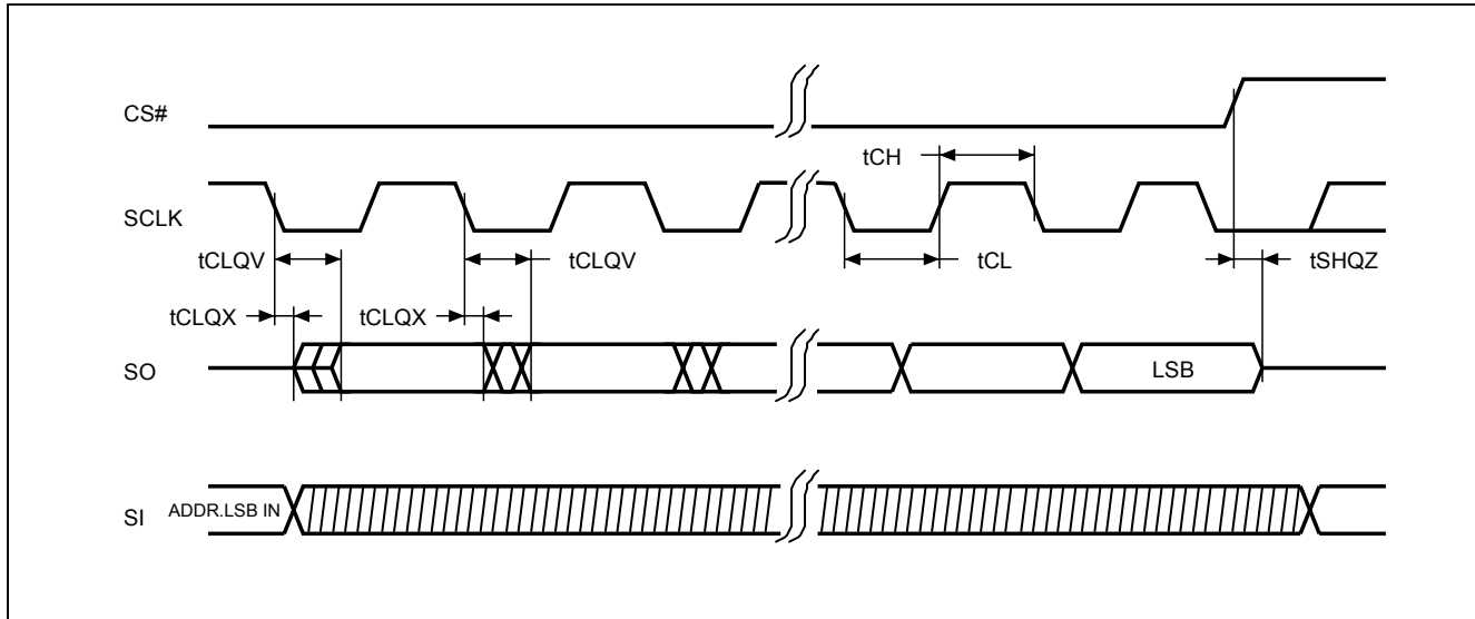
Figure 43. Output Timing
