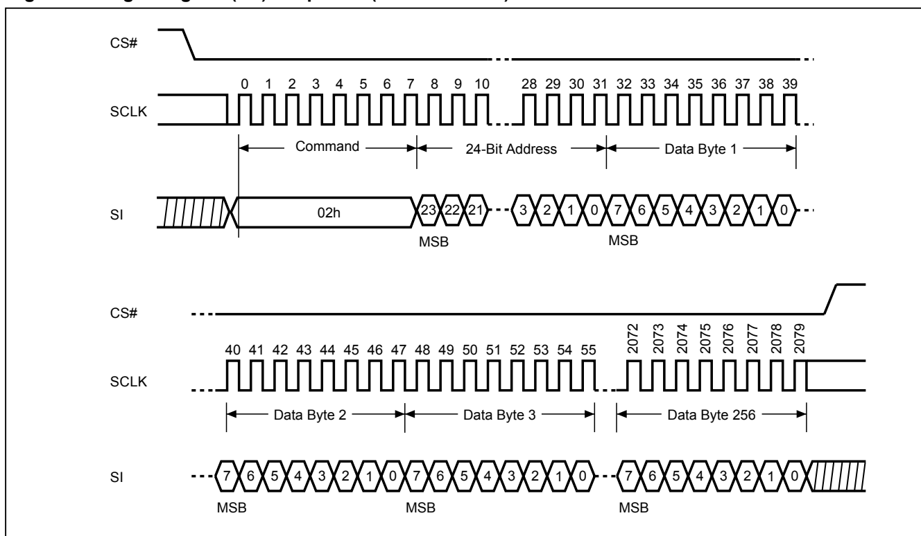
Figure 22. Page Program (PP) Sequence (Command 02h)
