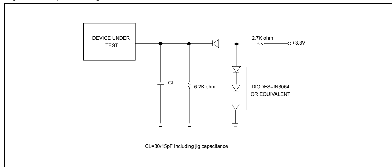
Figure 41. Output Loading
