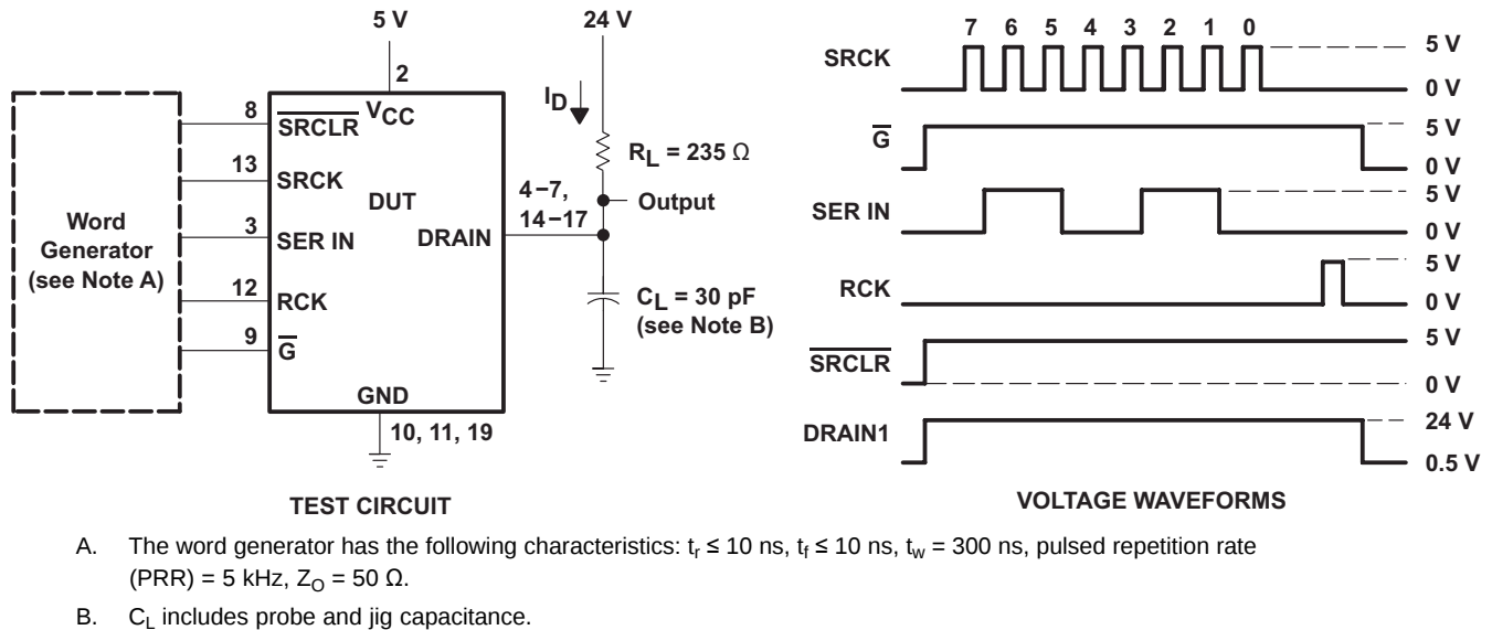
Figure 8. Resistive-Load Test Circuit and Voltage Waveforms
