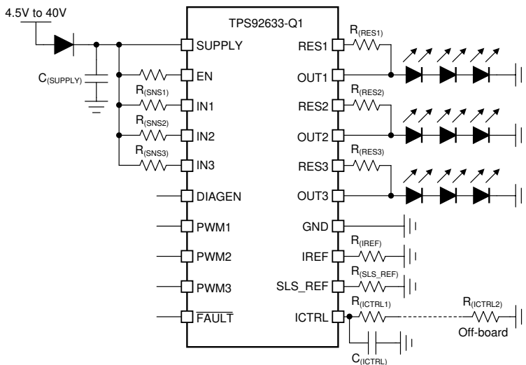
图 7-1. Application Schematic For Off-Board Brightness Binning Resistor
