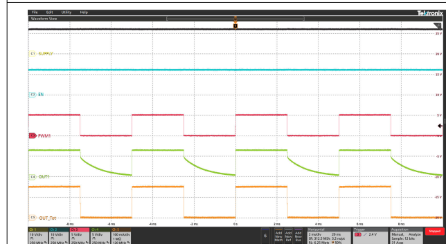
Ch1 = V_{(SUPPLY)} Ch2 = V_{(EN)} Ch3 = V_{(PWM1)} Ch4 = V_{(OUT1)} Ch5 = I_{(OUT\_Tot)}
