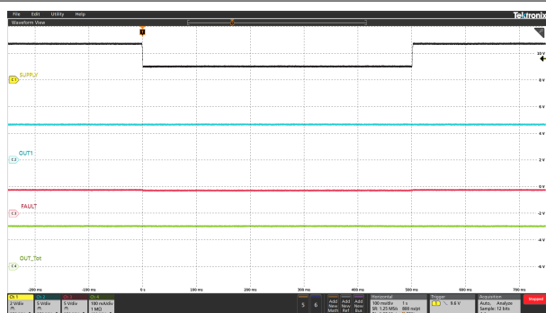
图 6-15. Single LED Short-Circuit Protection
