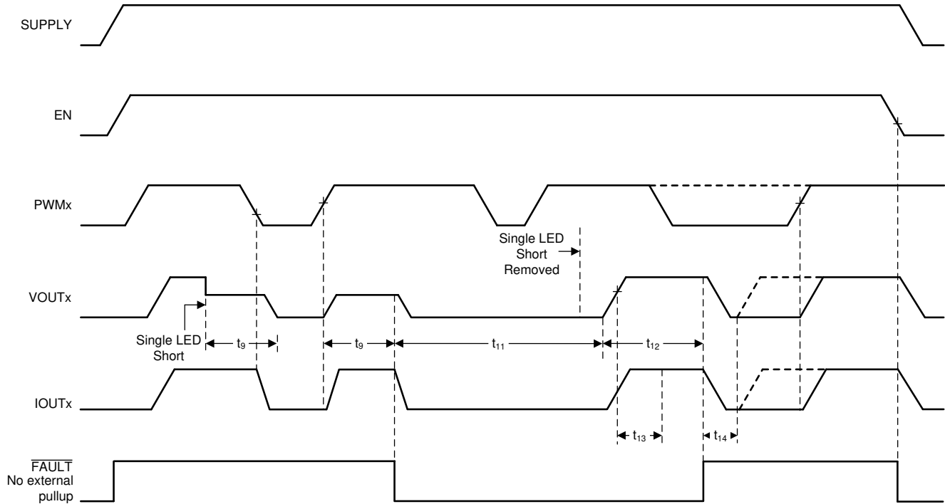
图 7-10. Single LED Short-Circuit Detection and Recovery Timing Diagram
