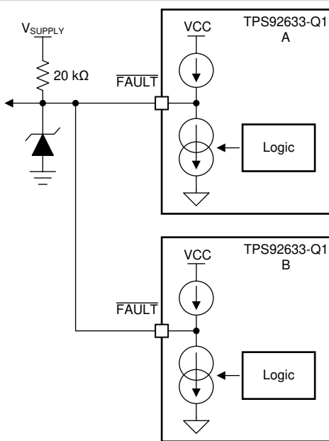
图 7-12. FAULT Bus For One-Fails-All-Fail Application
