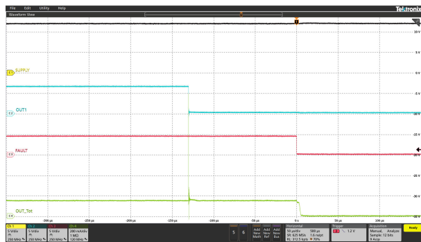
图 6-13. LED Short-Circuit Protection
