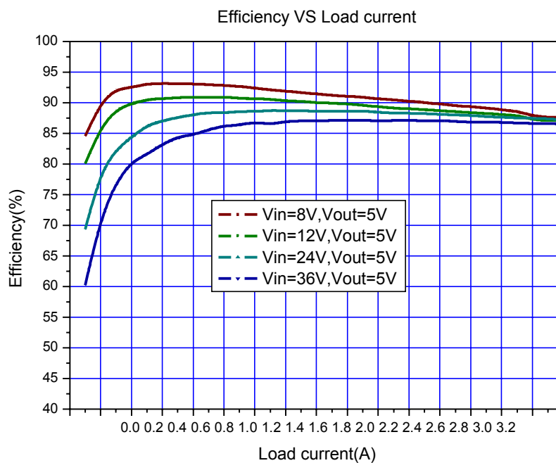
Figure7. XL2013 System Efficiency Curve
