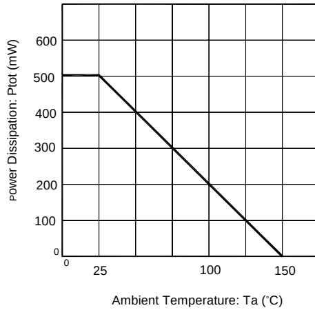
Fig.1 P_{tot} - T_a
