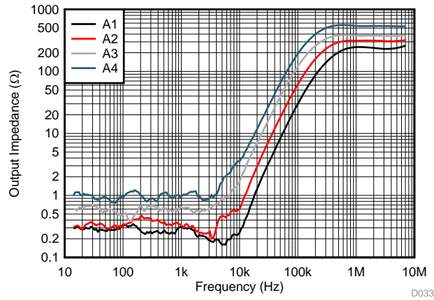
图 37. Output Impedance vs Frequency
