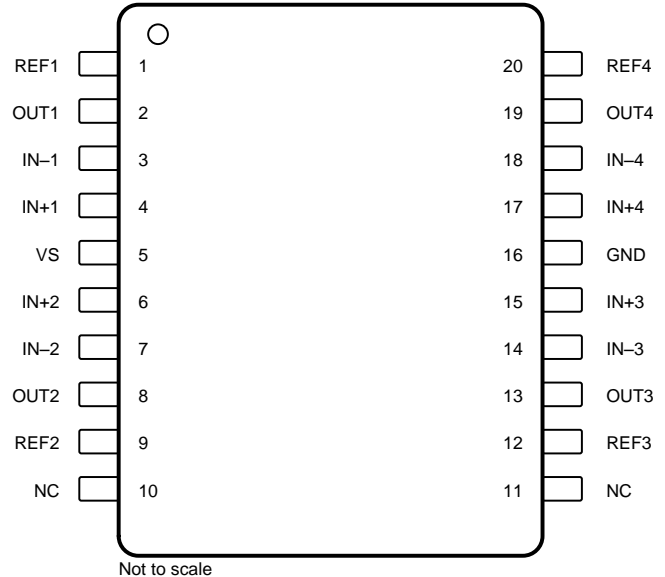
INA4181: PW Package 20-Pin TSSOP Top View
