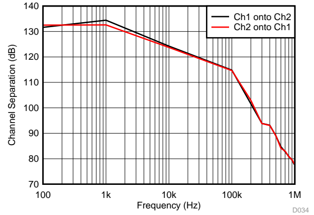
图 38. Channel Separation vs Frequency (INA2181)
