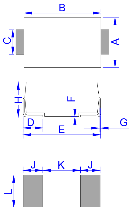
DO-214AA (SMB)
