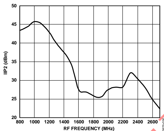
Figure 17. IIP2 vs. F_{RF} , V_{VGIN} = 1.2 V, Baseband Tone1 = 5 MHz, -10 dBm, Baseband Tone2 = 6 MHz, -10 dBm, Temperature = 25°C, V_S = 5 V
