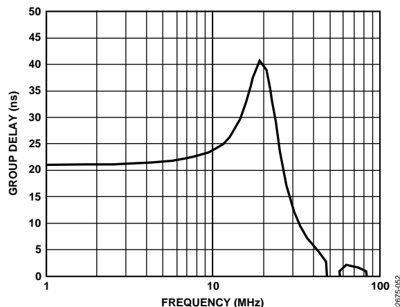
Figure 52. Group Delay of 20 MHz Baseband Low-Pass Filter
