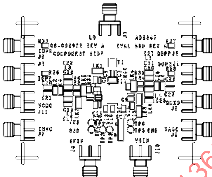
Figure 54. Silkscreen of Component Side
