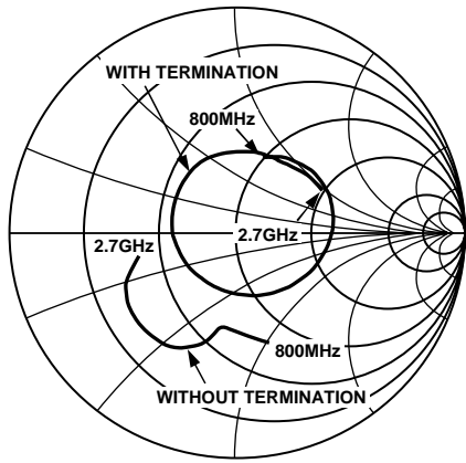
Figure 33. S11 of LOIN vs. F_{LO} , V_{GIN} = 0.7\text{ V} , V_S = 5\text{ V}
