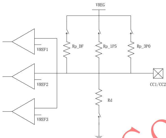
Pull-up/Pull-down Resistor
