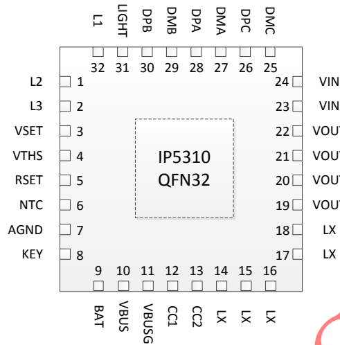
Fig 2 IP5310 Pin Diagram
