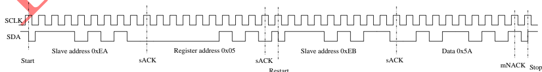
I2C Read
