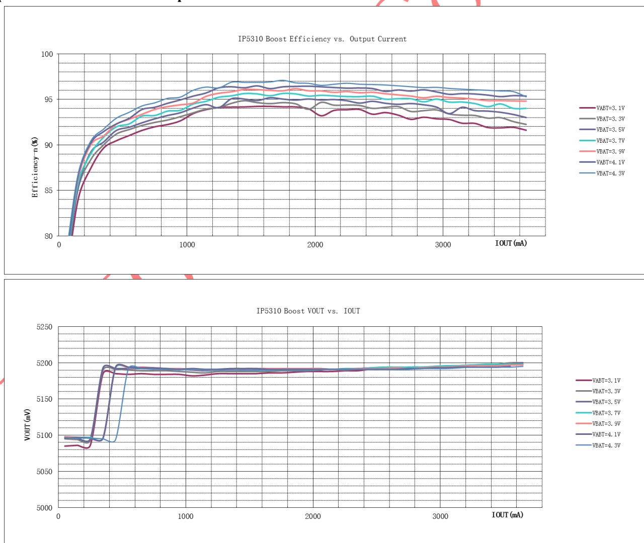
Fig 4 IP5310 Boost Efficiency and VOUT Vs. IOUT
